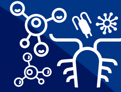
Carbon-Plankton Dynamics
