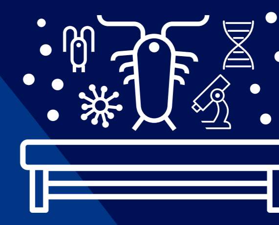
Ecosystem-level EOVs
