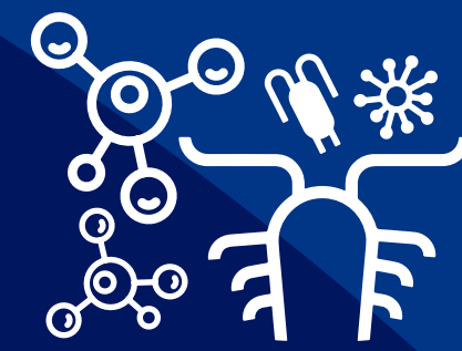
Carbon-Plankton Dynamics
