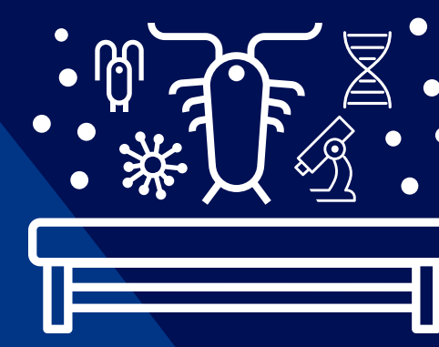
Ecosystem-level EOVs
